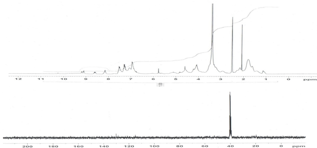
Figure 2. ^1\text{H} and ^{13}\text{C} NMR spectra of compound 9 in \text{D}_2\text{O} solution
