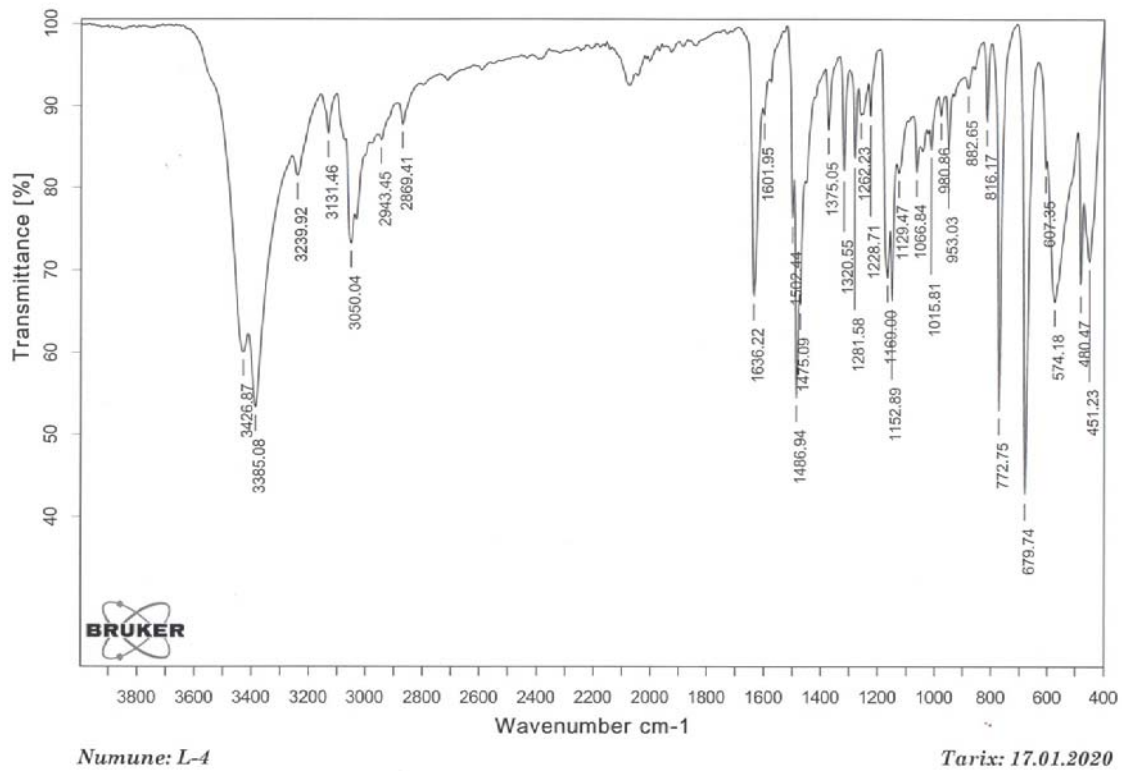
Figure 8. FTIR spectrum of compound 11
