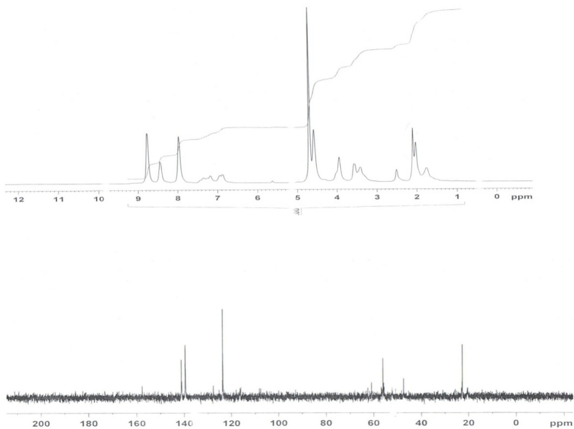
Figure 3. ^1\text{H} and ^{13}\text{C} NMR-spectra of compound 10 in \text{D}_2\text{O} solution
