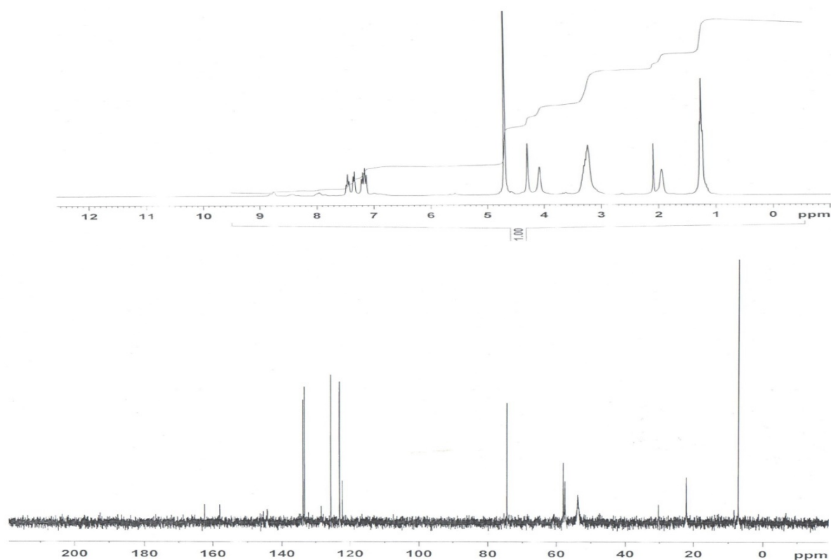
Figure 1. 1 H and 13 C NMR spectra of compound 8 in D 2 O solution
