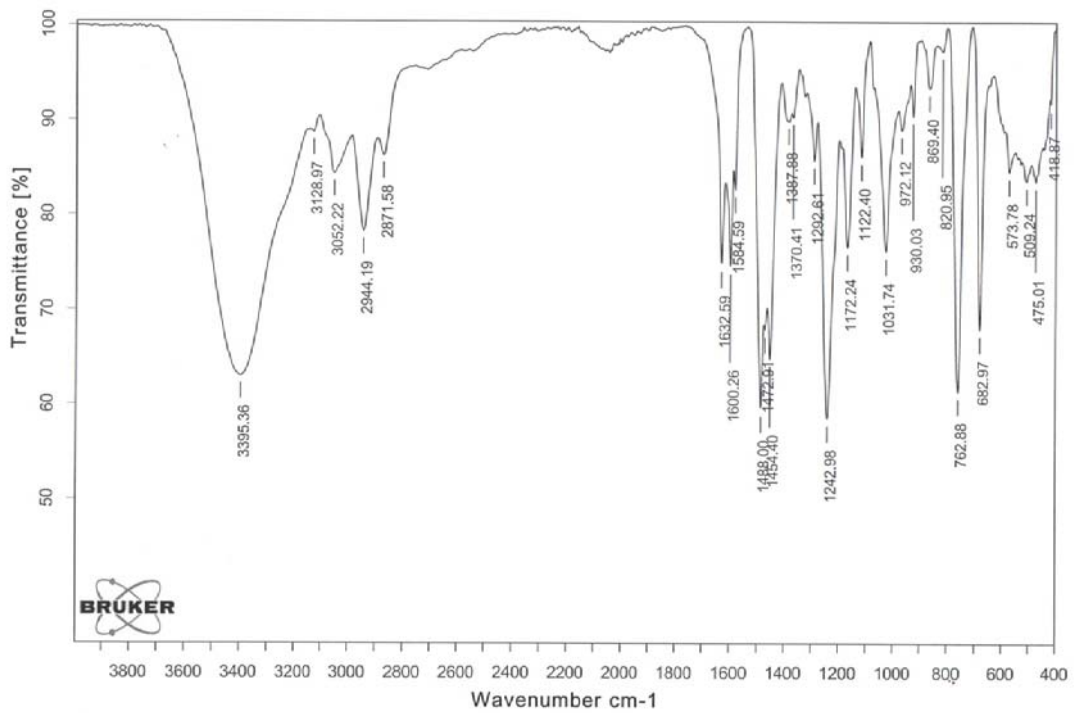
Figure 7. FTIR spectrum of compound 10
