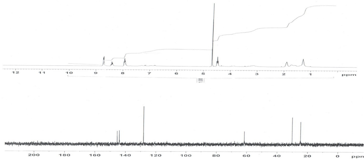
Figure 4. ^1\text{H} and ^{13}\text{C} NMR-spectra of compound 11 in \text{D}_2\text{O} solution
