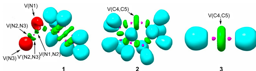
Fig. 1 — MPWB1K/6-311G(d,p) ELF localisation domains represented at an isosurface value of ELF = 0.81 of benzyl azide 1 , cyclooctyne 2 , and acetylene 3 . Protonated basins are shown in blue, disynaptic basins are shown in green, monosynaptic basins are shown in red and core basins are shown in magenta colours
