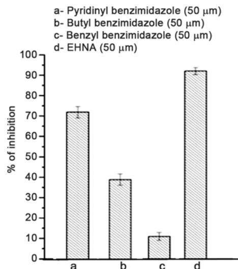
Figure 5 — ADA inhibitory activity of Zn 394330 (a), Zn 2475956 (b), Zn 132982 (c) and standard inhibitor EHNA (d).
