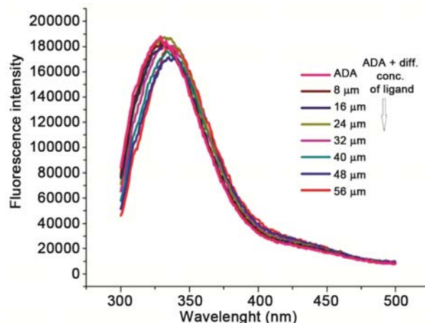
Figure 10 — Fluorescence emission spectra of ADA with increasing concentration of Zn 132982 (8–56 \mu\text{M} ) on excitation at 280 nm
