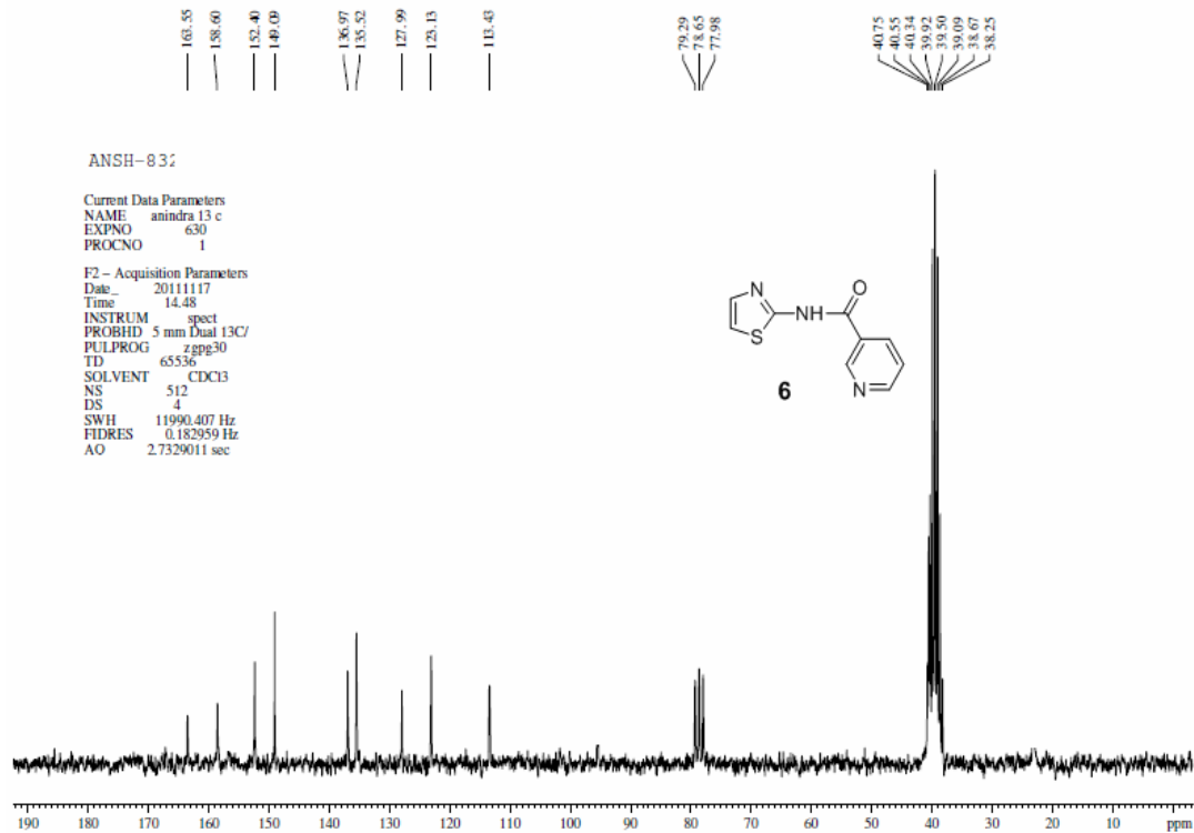
Figure S11. ^{13}\text{C} NMR spectrum of compound 6
