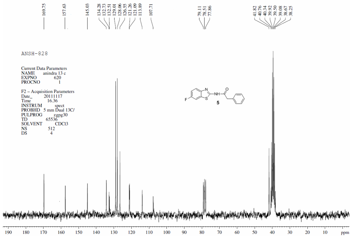
Figure S10. ^{13}\text{C} NMR spectrum of compound 5
