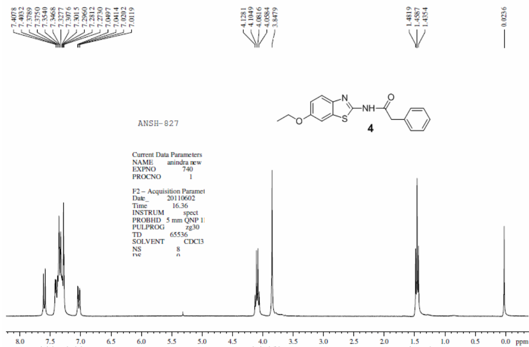
Figure S7. ^1\text{H} NMR spectrum of compound 4
