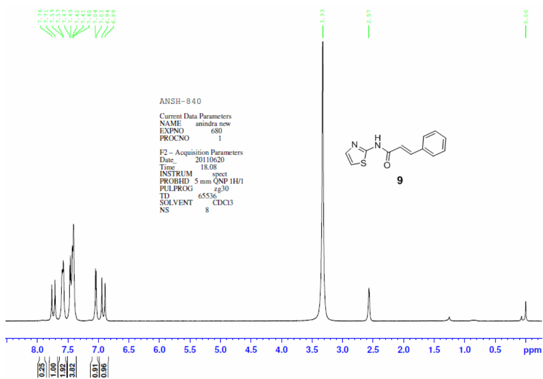
Figure S16. ^1\text{H} NMR spectrum of compound 9
