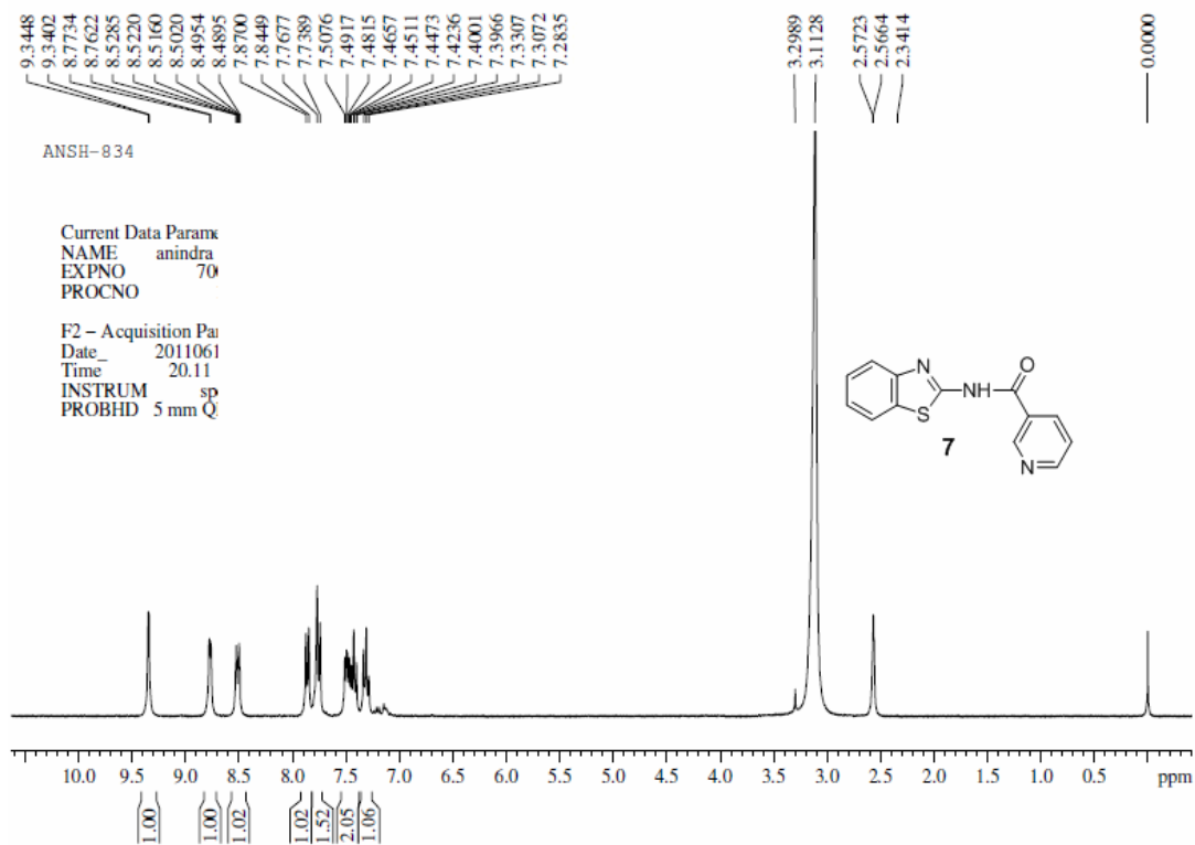
Figure S12. ^1\text{H} NMR spectrum of compound 7
