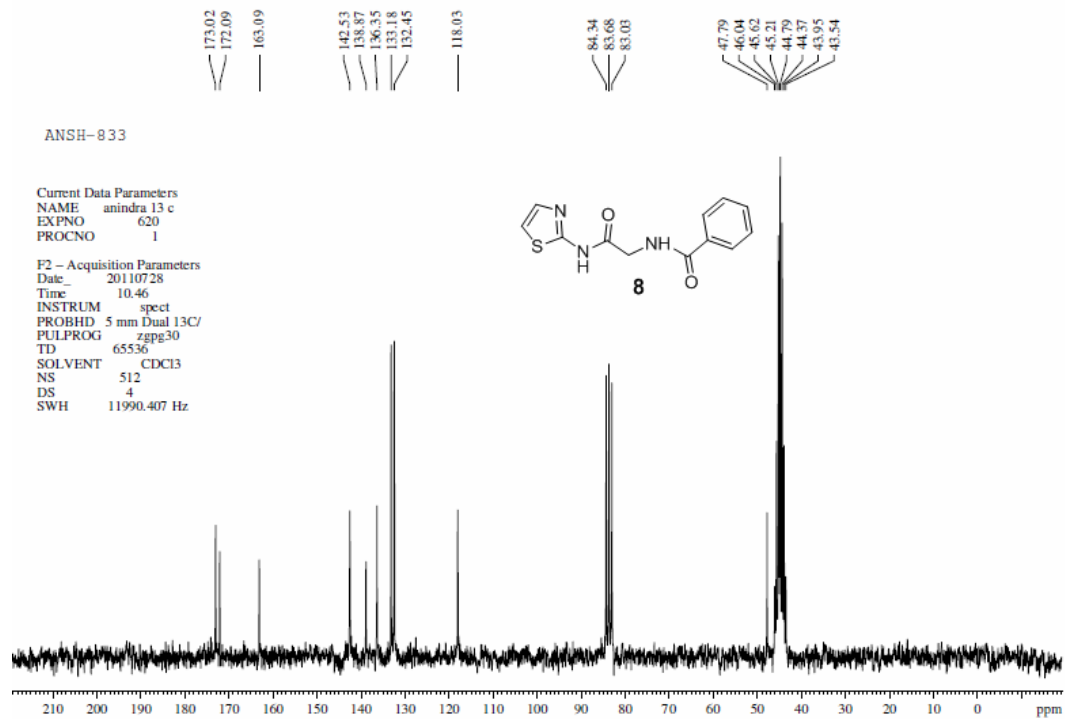
Figure S15. ^{13}\text{C} NMR spectrum of compound 8
