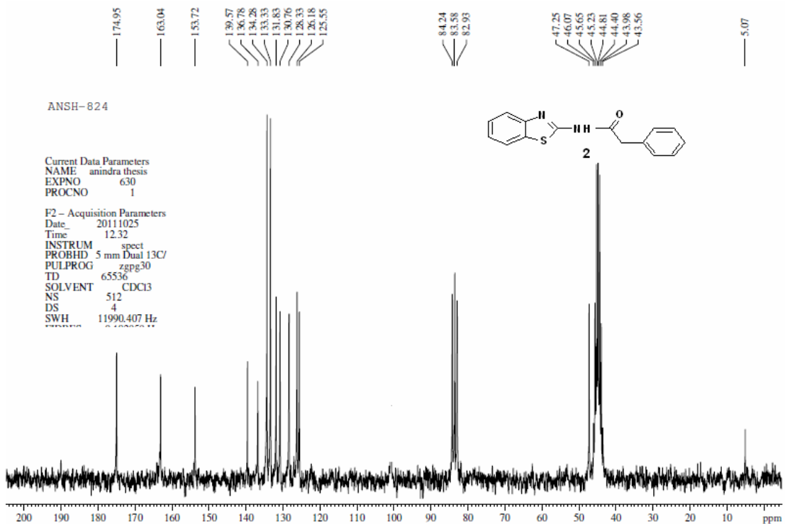
Figure S4. ^{13}\text{C} NMR spectrum of compound 2
