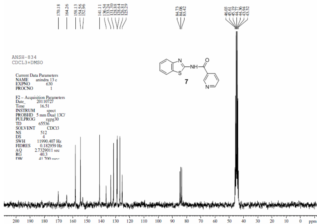
Figure S13. ^{13}\text{C} NMR spectrum of compound 7
