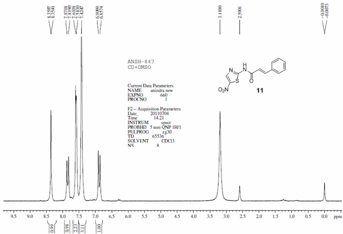
Figure S17. ^1\text{H} NMR spectrum of compound 11
