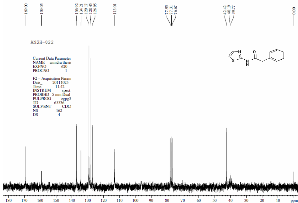
Figure S2. ^{13}\text{C} NMR spectrum of compound 1
