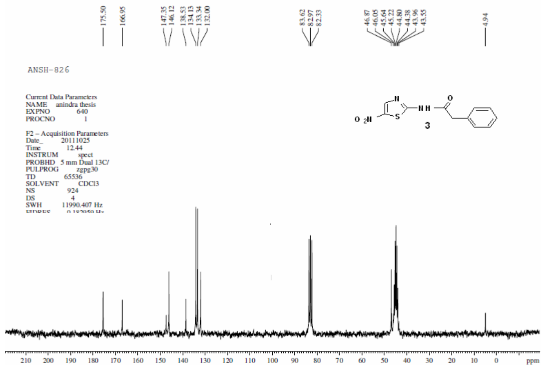
Figure S6. 13 C NMR spectrum of compound 3
