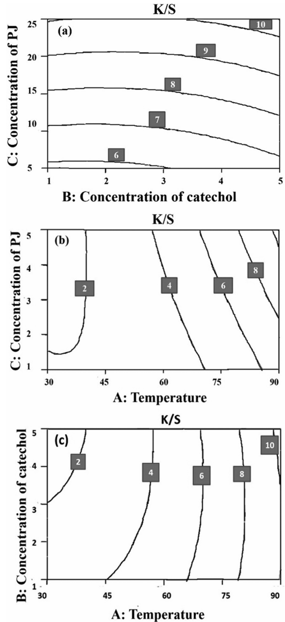
Fig. 4 — Selected contour plots obtained from RSM (a) Temperature – 90°C, (b) Concentration of catechol – 5%, and (c) Concentration of potato juice – 25%.
