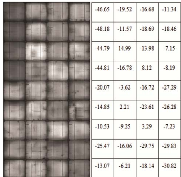
Fig. 7 — EL image and individual cell performance (%) of the 11 years aged D type PV module.
