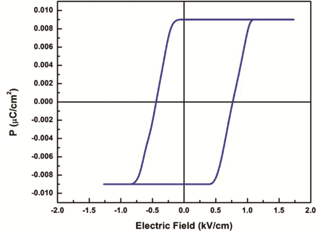
Fig. 5 – P-E loop for LTGO at room temperature.
