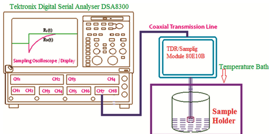
Fig. 1 — Experimental setup of time domain reflectometry.
