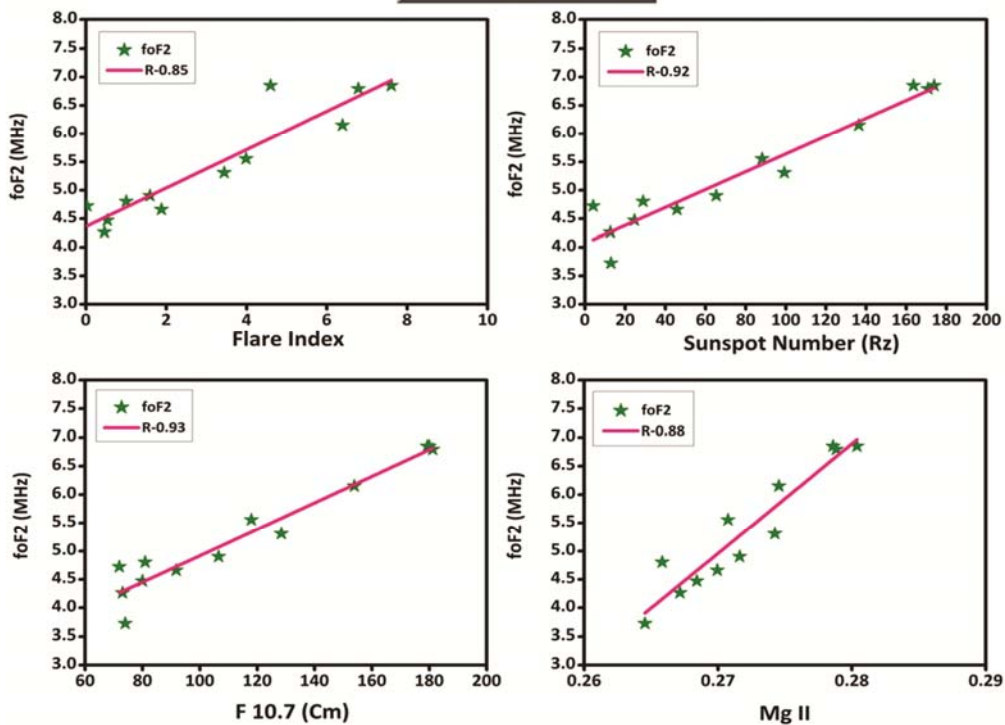
Fig. 12 — Scatter and Correlation of foF2 with flare index, sunspot number, F10.7 Cm and Mg II core to wing ratio during the solar cycle 23.
