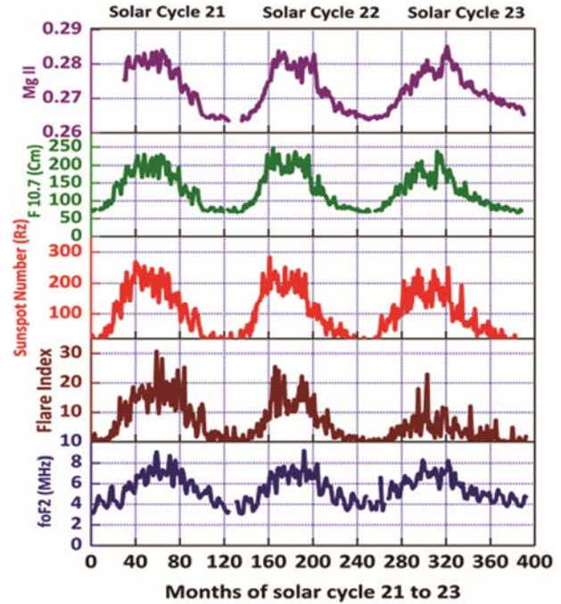
Fig. 13 — Cycle to cycle variation of foF2 with solar indices during solar cycle 21, 23 and 23.
